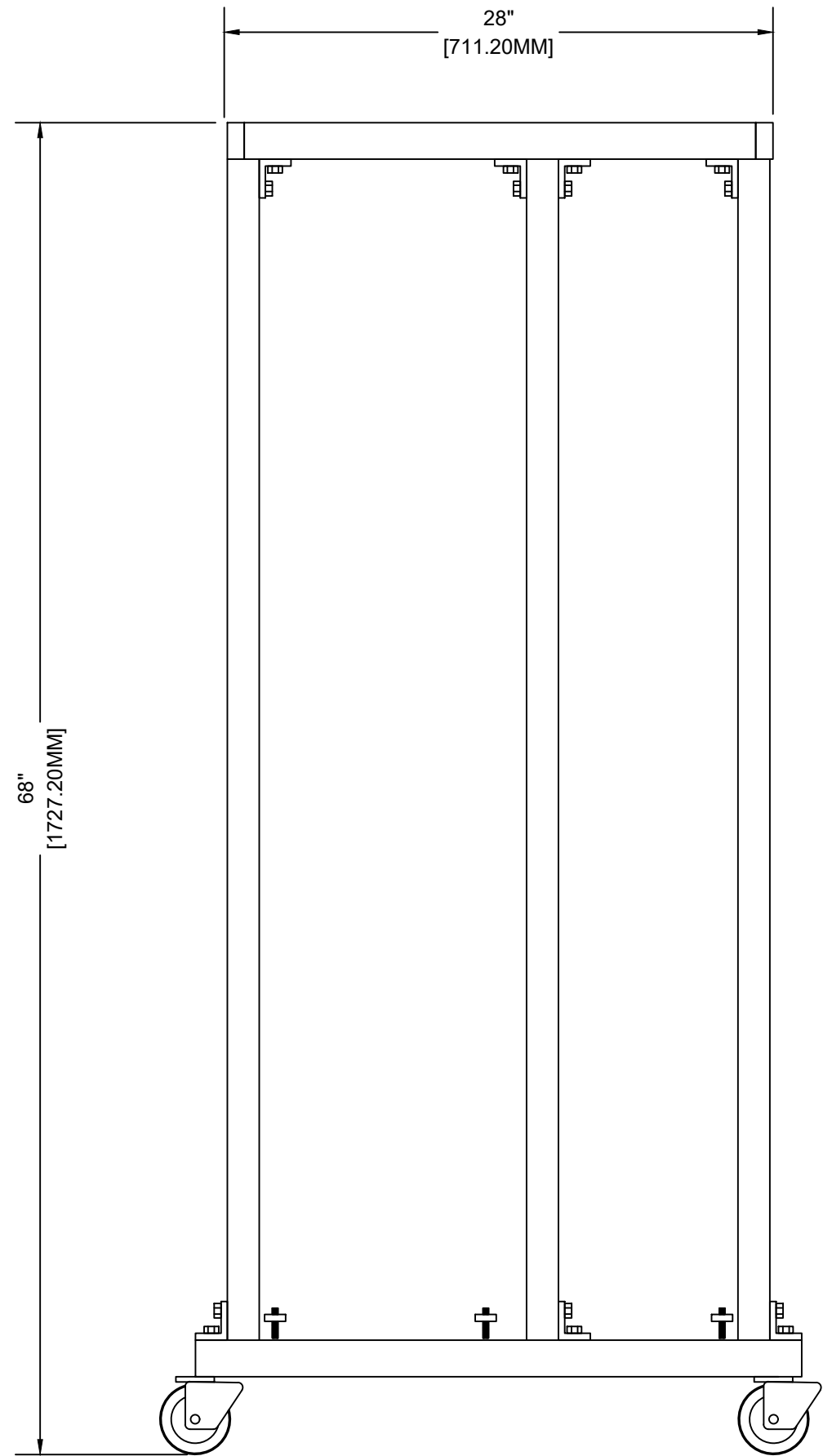
SIDE VIEW
