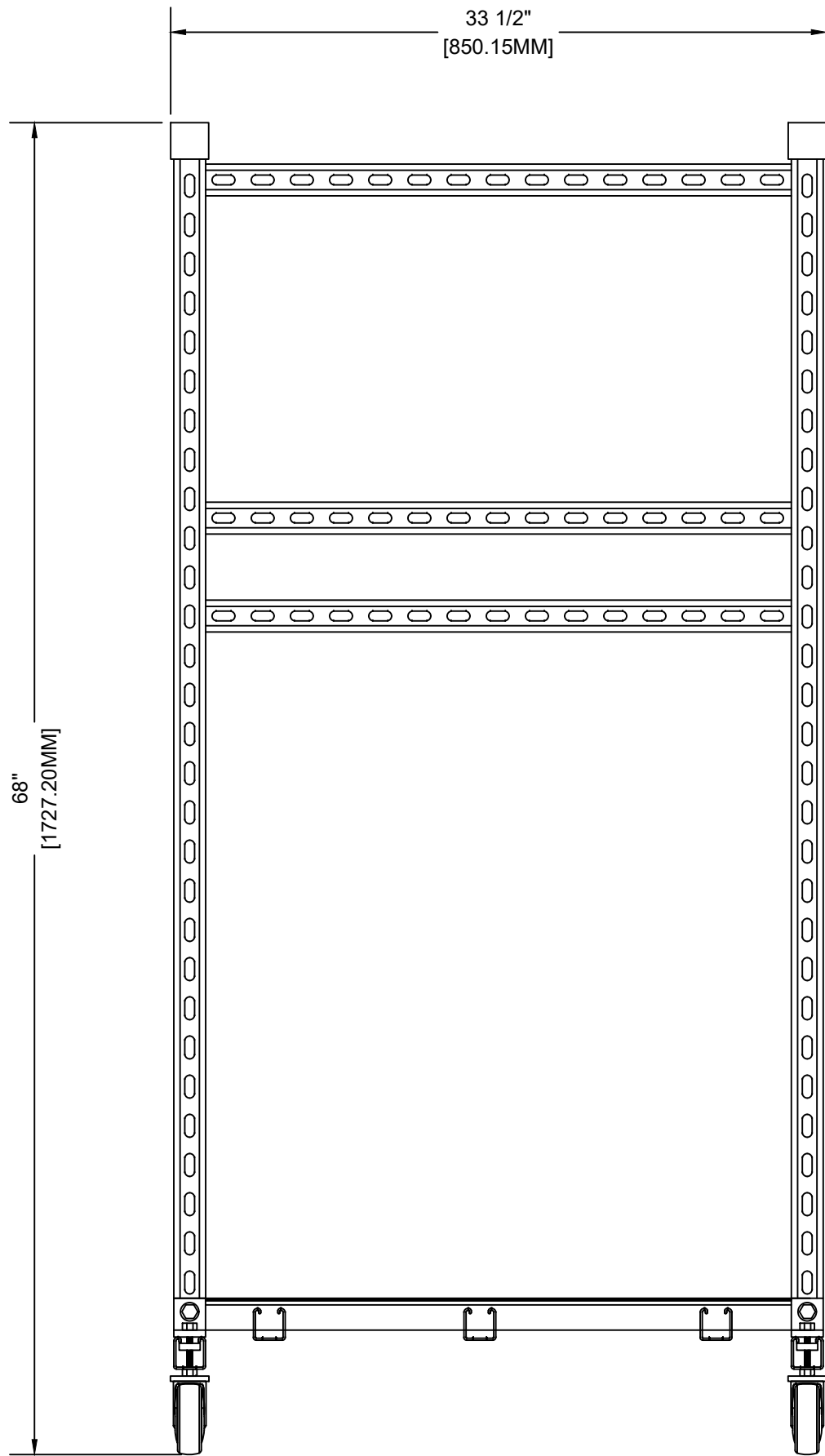
FRONT VIEW
