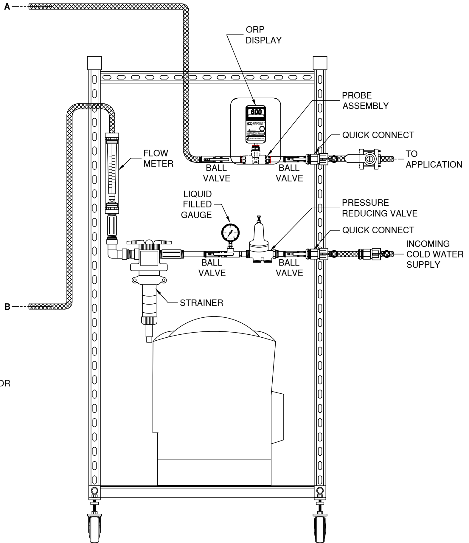
REAR VIEW
