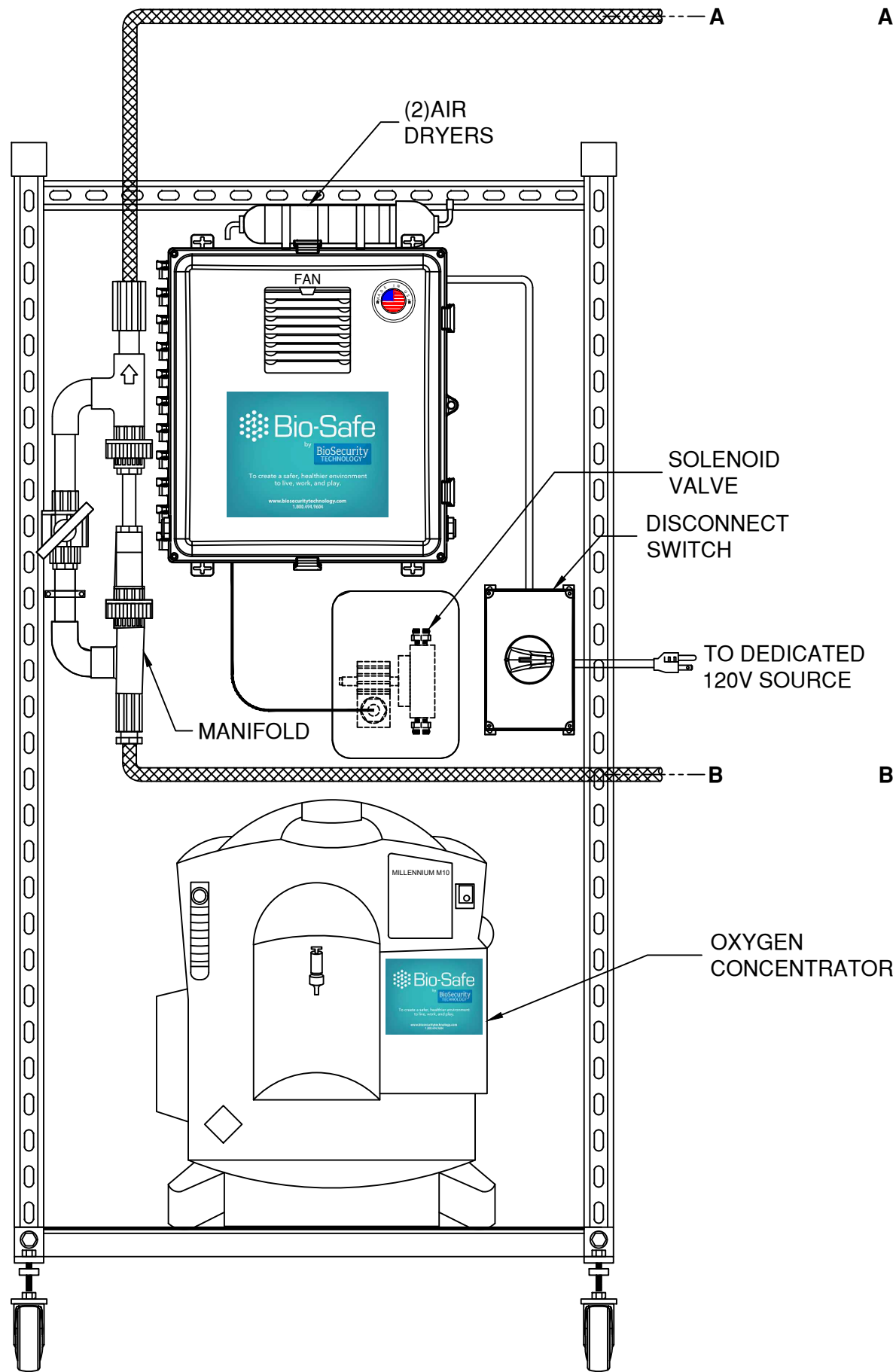
FRONT VIEW
