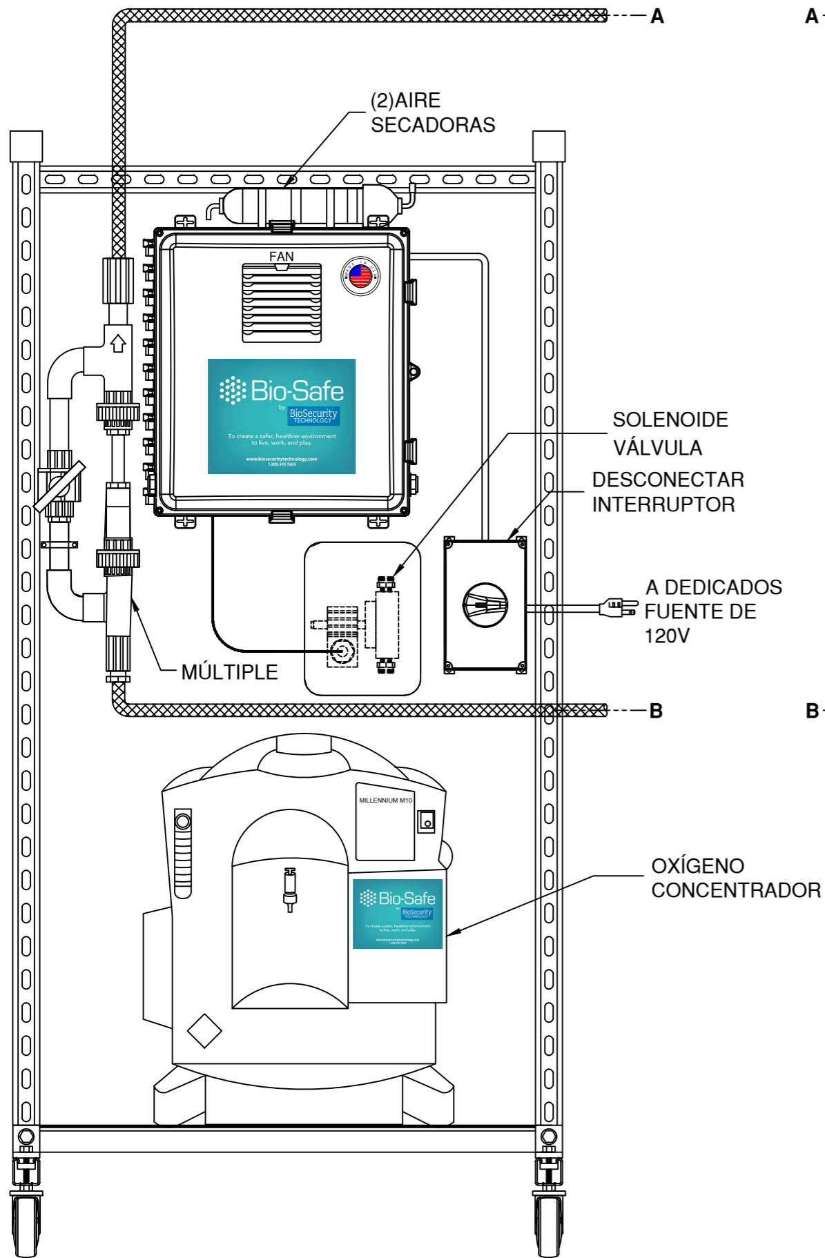
VISTA FRONTAL
