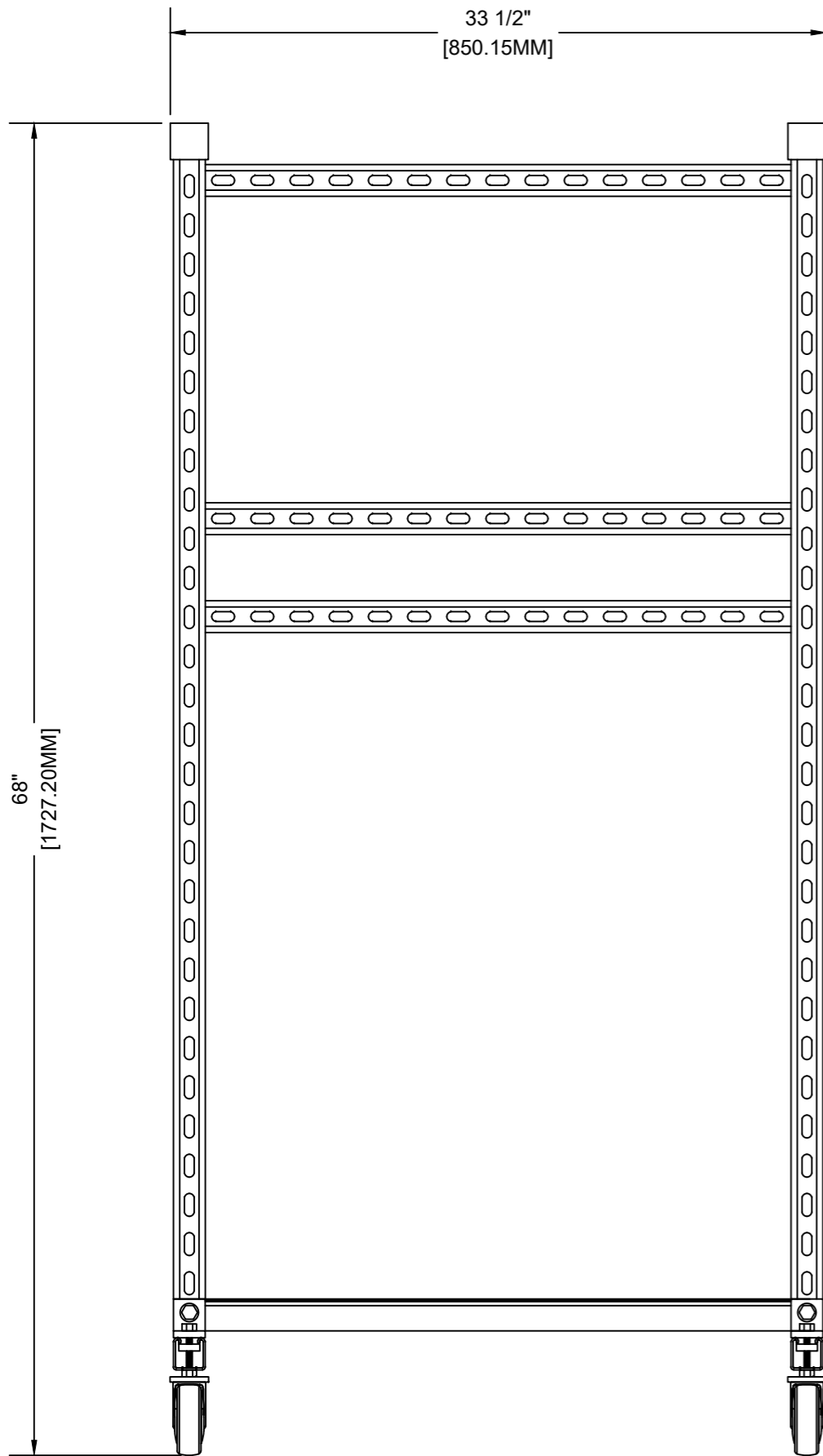
VISTA FRONTAL
